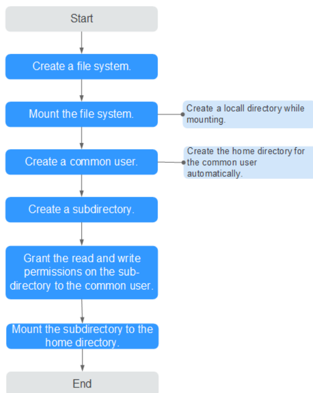
Figure 4-1 Flowchart
